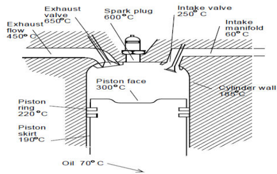
Fig 2 boundary conditions
