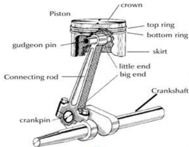
Fig 1 Piston Assembly
