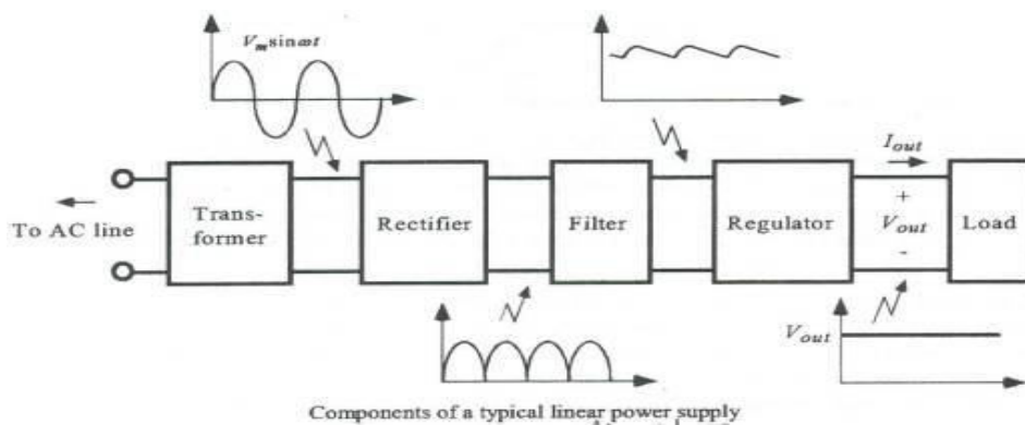
Fig. 4 Block diagram of the power supply.
