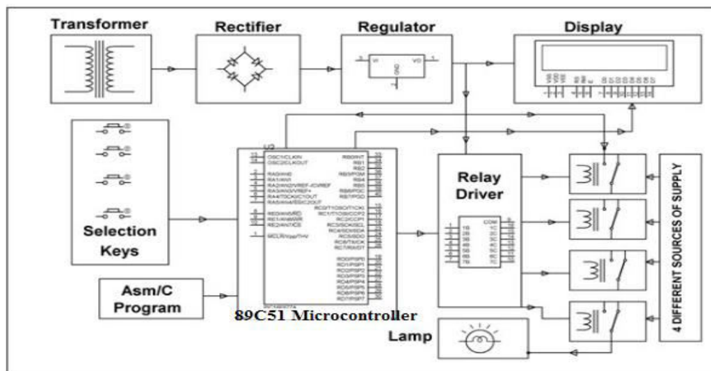
Fig. 1 Block diagram of the overall proposed system
