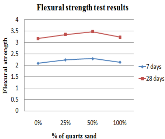
Graph 2: Flexural Strength of Concrete beams with various percentages of Quartz sand
