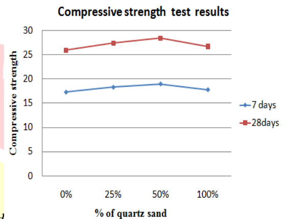
Graph 1: Compressive Strength of Concrete Cubes with various percentages of Quartz
