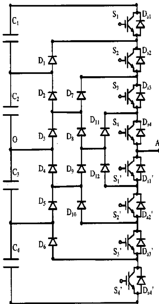
Fig 3: Improved Diode clamped Inverter
