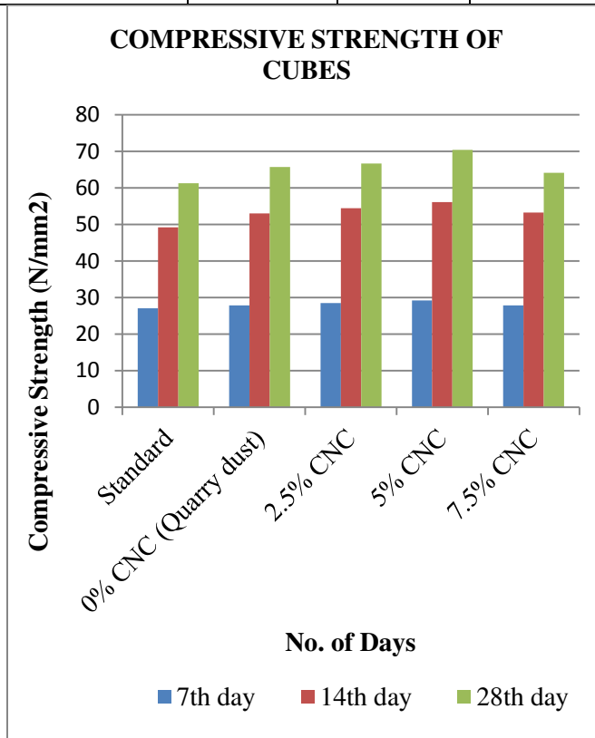
Fig.4.1. Comparison of compressive strength between standard, 0% CNC (Quarry dust), 2.5%, 5% and 7.5% CNC concrete cubes
