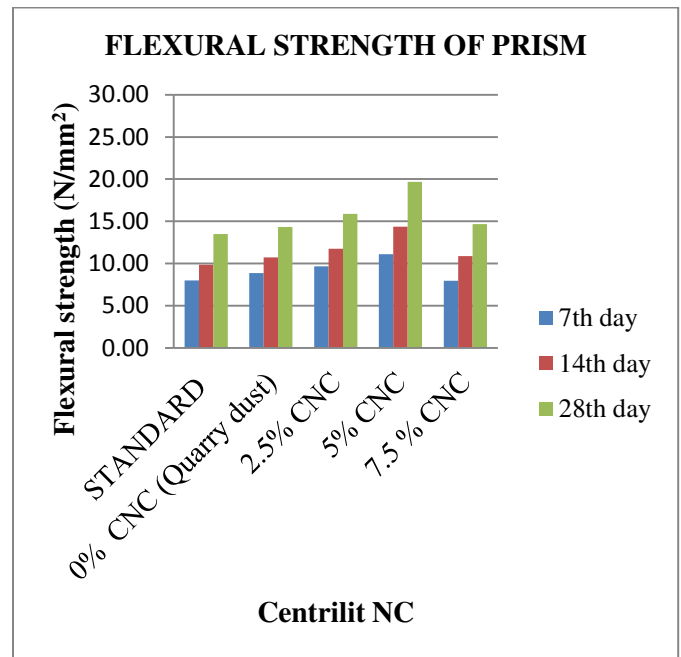
Fig.4.3. Comparison of flexural strength between standard, 0% CNC (Quarry dust), 2.5%, 5% and 7.5% CNC concrete prisms
