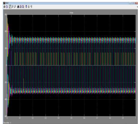
Fig 4. Three phase output from hydro and Solar
