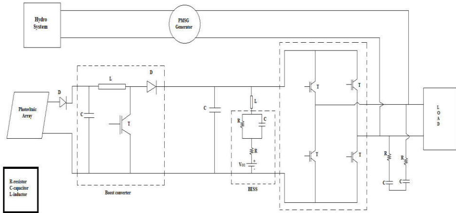
Schematic diagram of HYDRO-SOLAR HYBRID SYSTEM
