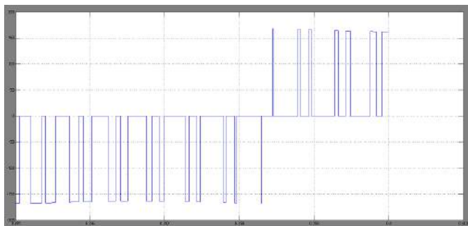
Fig.6 output voltage waveform for inverter
