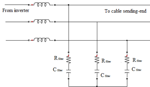
Fig.4 RLC filter at the inverter output
