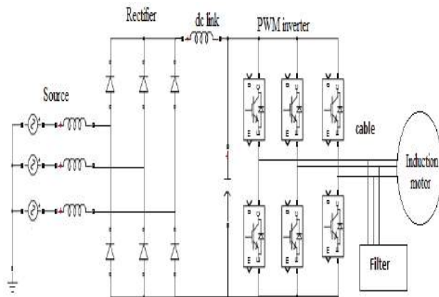
Fig.1 PWM inverter driving an induction motor with filter at the end of the cable.
