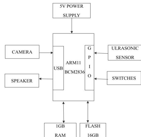
Figure 2: Block diagram of proposed assistive system
