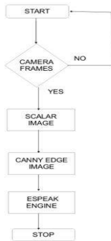
Figure 3: Flow chart for color identification system
