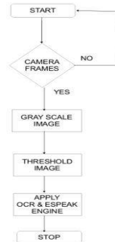
Figure 4: Flow chart for Text reading
