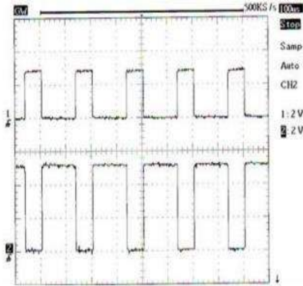
Fig. 9. PWM signals before and after optocouplers
