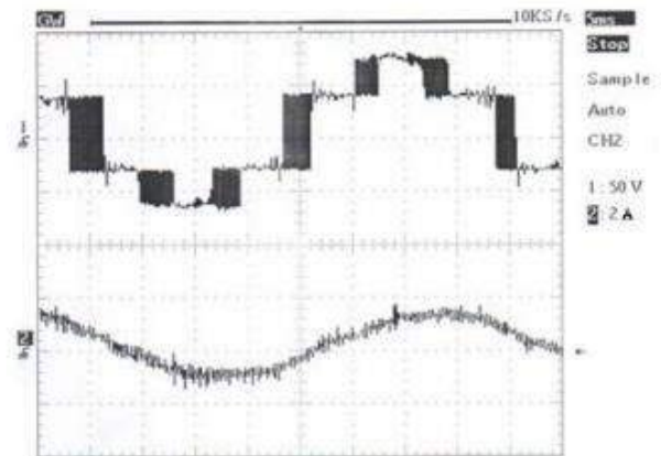
Fig. 11. Wave form of the phase voltage and current for f=25\text{Hz} with a load torque
