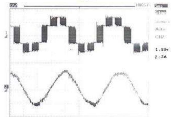
Fig. 11. Wave form of the phase voltage and current for f=25\text{Hz} with a load torque
