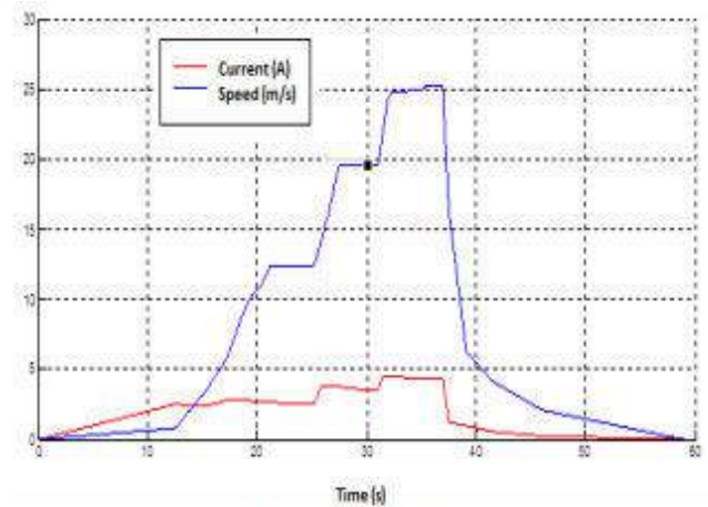
Fig. 13. Running the vehicle in flat road
