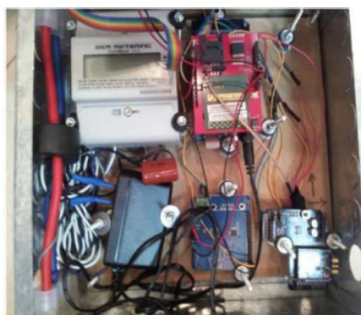
Figure 2. Components inside the steel box
