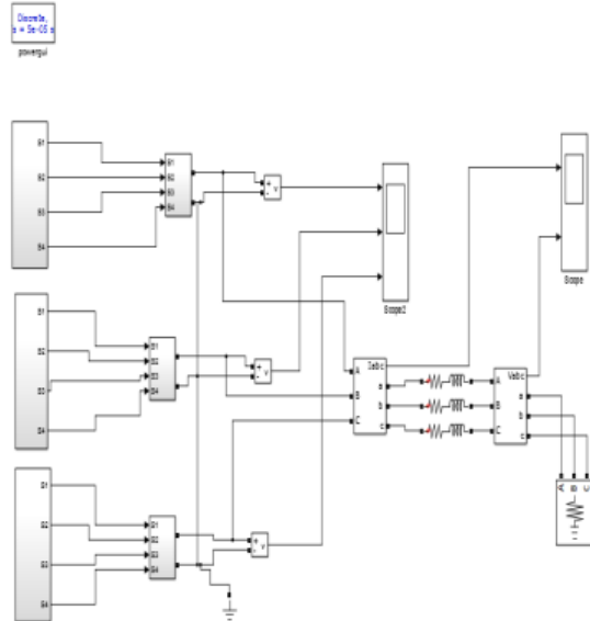
Fig. 5. Matlab/Simulink model of three phase cascaded multilevel inverter
