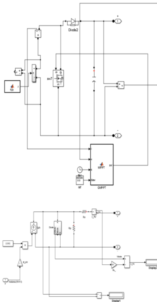
Fig. 10. PV Array with MPPT
