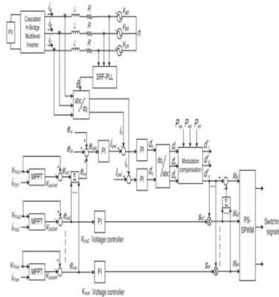
Fig. 3. Control scheme for three phase modular cascaded H-bridge multilevel PV inverter.
