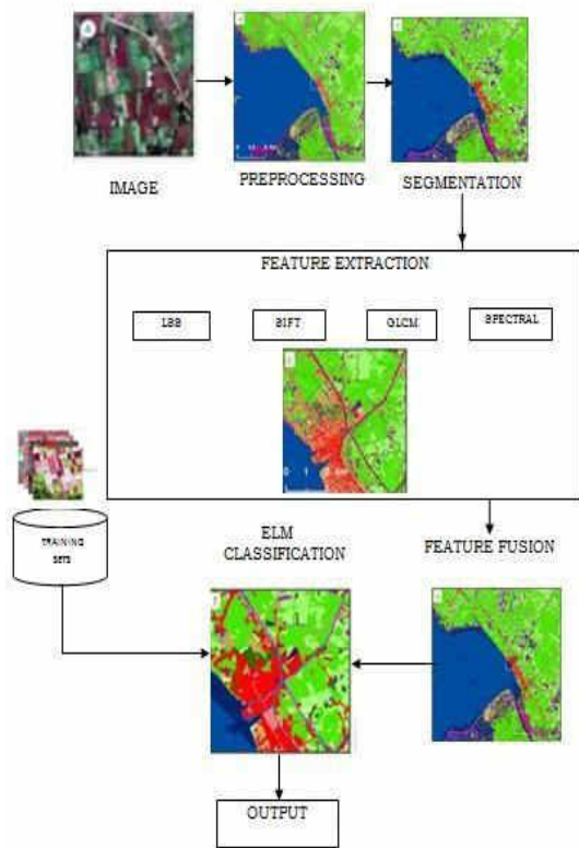
Fig.2 ELM Classification
