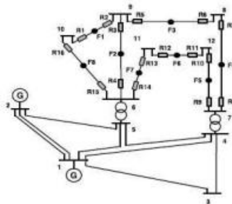
Fig 1.1. Single line diagram of the modified IEEE 14-bus system for protection coordination
