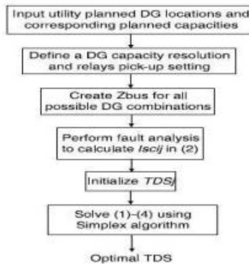
Fig 3.1 Flow chart of proposed system
