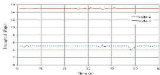
Fig. 9. Impact of CTS Packets Transmitted by the Coordinator Interface on FTP traffic (CTS parameters: Interval=10ms, NAV=5ms, Power=5dBm)
