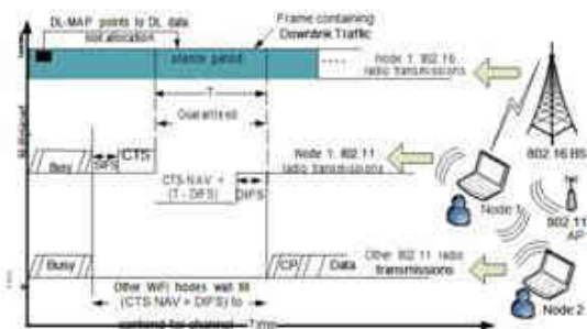
Fig. 5. Protecting WiMAX reception
