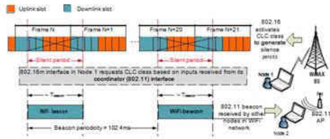
Fig. 6. Protecting WiFi reception
