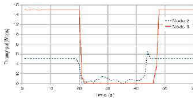
Fig. 8. Impact of CTS Packets Transmitted by the Coordinator Interface on FTP traffic (CTS parameters: Interval=1 ms, NAV=5 ms, Power=5 dBm)
